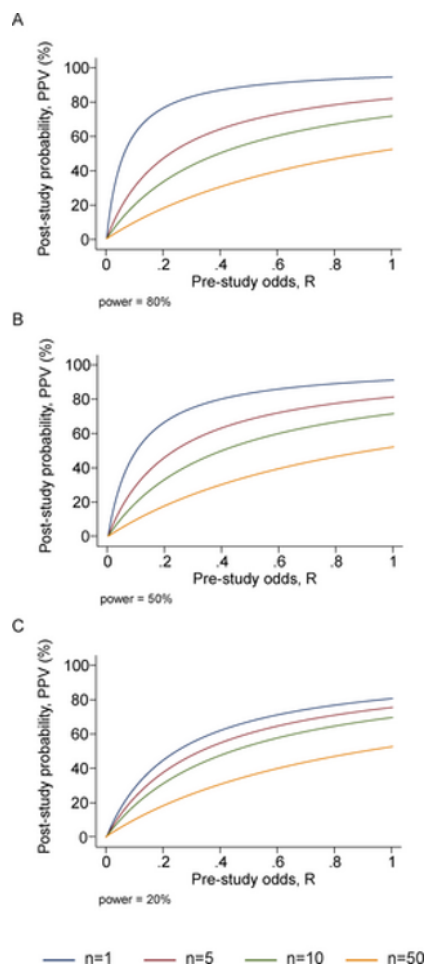
Figure 2. PPV (Probability That a Research Finding Is True) as a Function of the Pre-Study Odds for Various Numbers of Conducted Studies, n . Panels correspond to power of 0.20, 0.50, and 0.80. https://doi.org/10.1371/journal.pmed.0020124.g002
