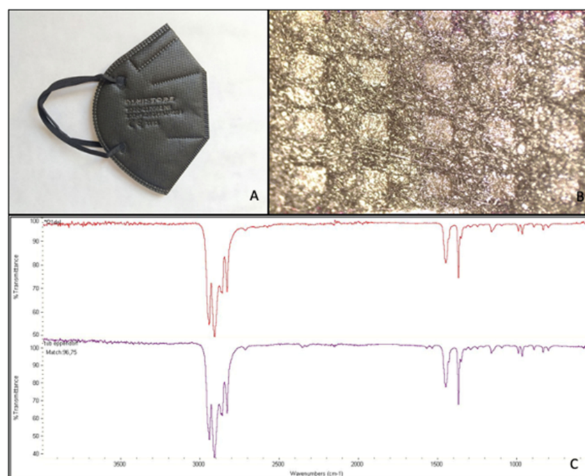
Figure 3. Facial mask FFP2 N studied (A); structure after disassembling in layers (500 \mu\text{m} scale bar) (B); and mask spectrum (at the top), spectrum listed in the library (at the bottom) identifying polypropylene, atactic, 96.75% (C).
